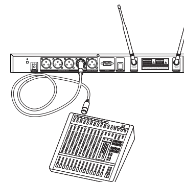
4. Connect Receiver with Audio System
