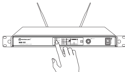
6. Press the channel key one by one, then press the function operation knob to enter the single channel menu settings, find out AFS, and scan out the non-interference frequency
