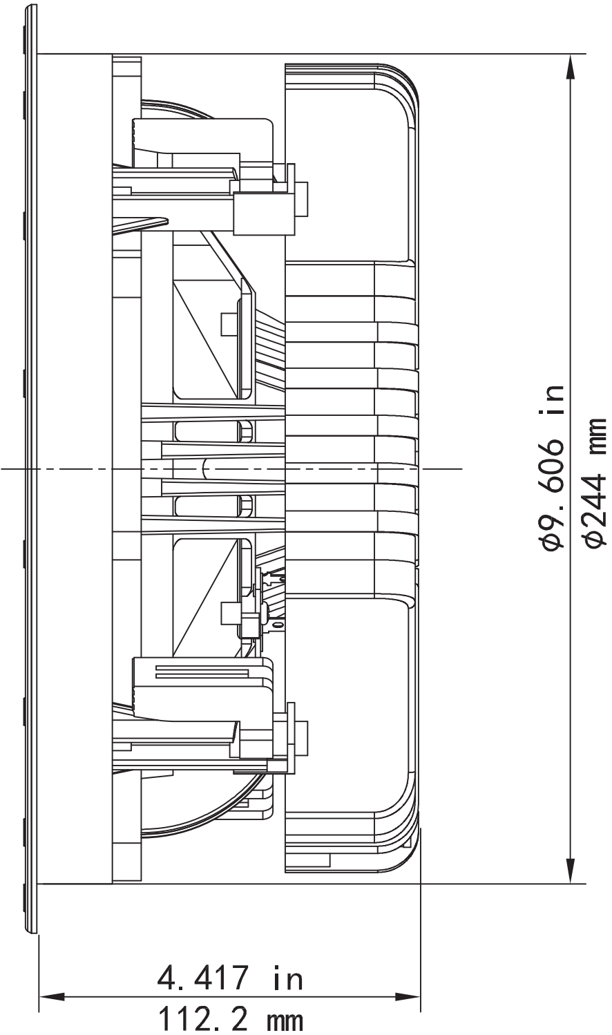
MOUNTING DEPTH/ MINIMUM CUTOUT
