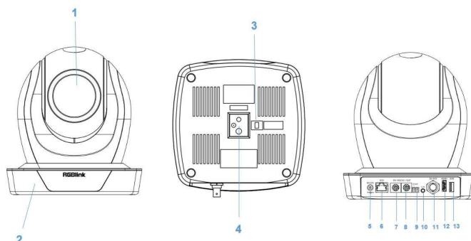
Figure 2.1 Camera Interface
